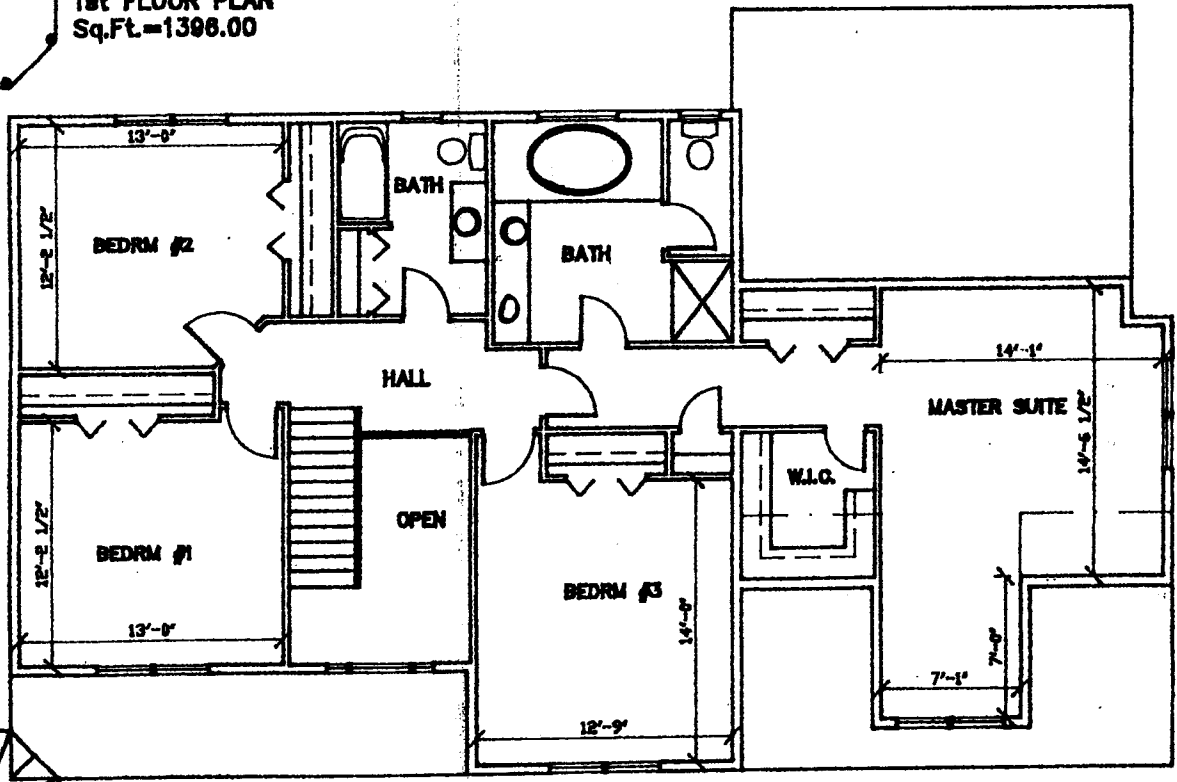
2nd FLOOR PLAN Sq.Ft.=1357.00
