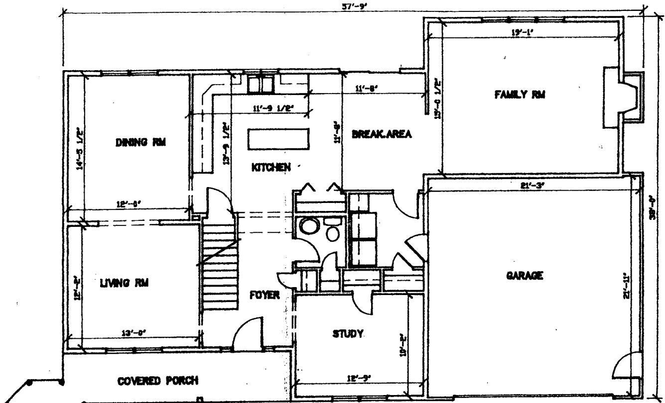
1st FLOOR PLAN Sq.Ft.=1398.00
